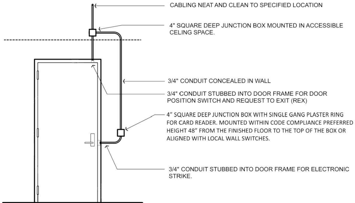
TYPICAL SINGLE CARD READER CONTROLLED DOOR SCALE: NONE
