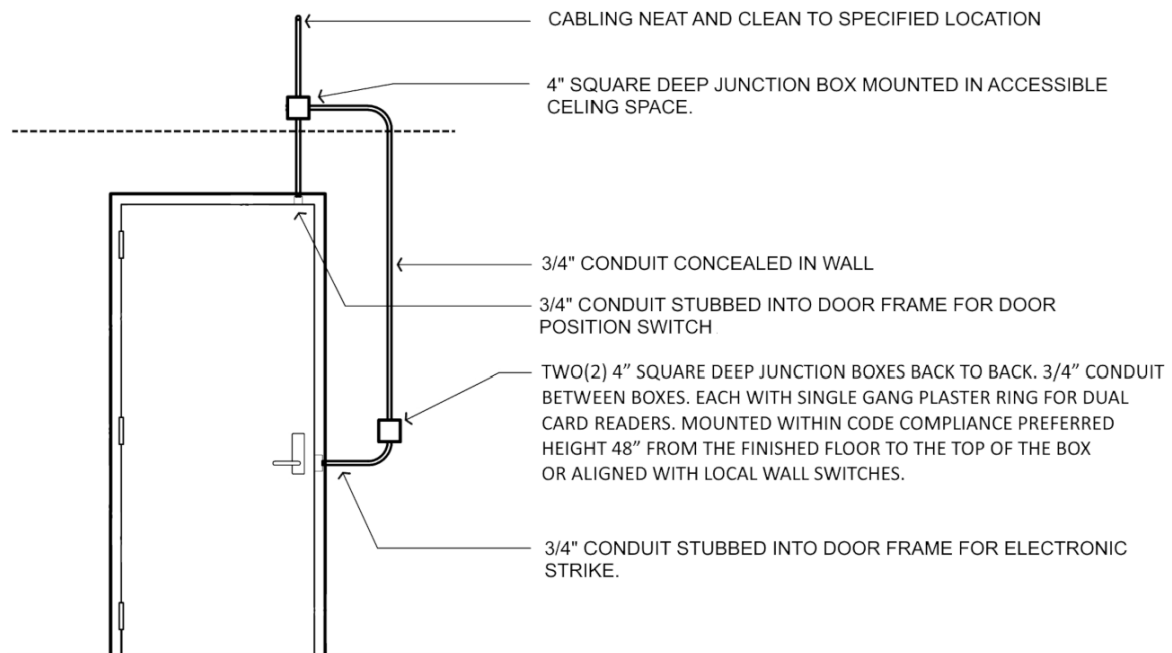
TYPICAL DUAL CARD READER CONTROLLED DOOR SCALE: NONE
