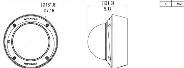
Dome Camera with Surface Mount (H6A Dome camera + provided surface mount)
